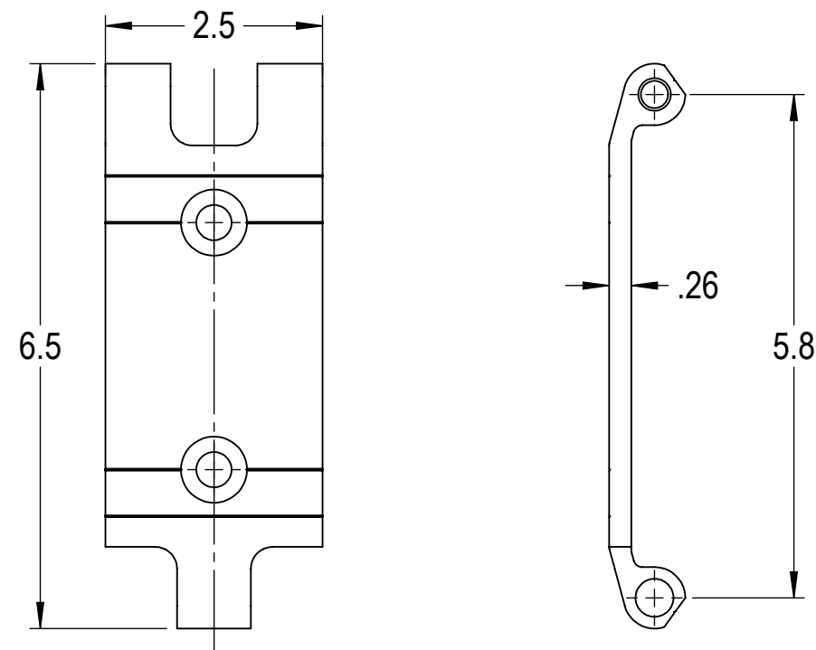
7 INTERMEDIATE END HINGE DETAIL
