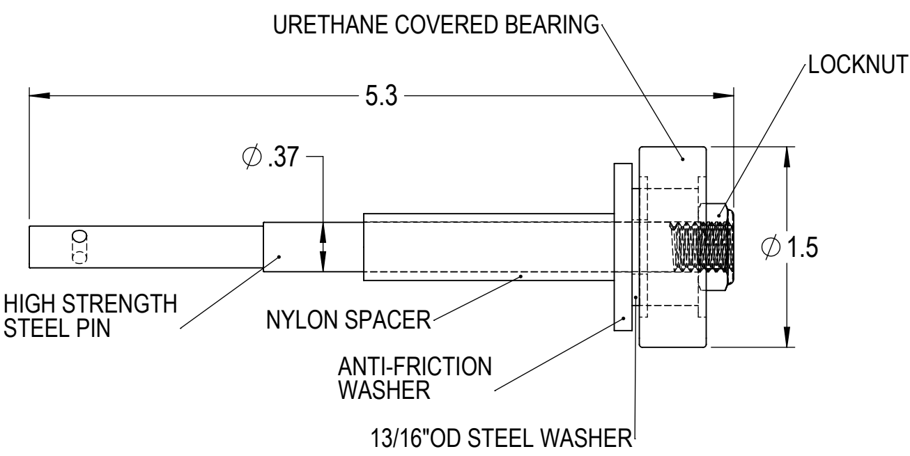
6 SLAT ROLLER ASSEMBLY
