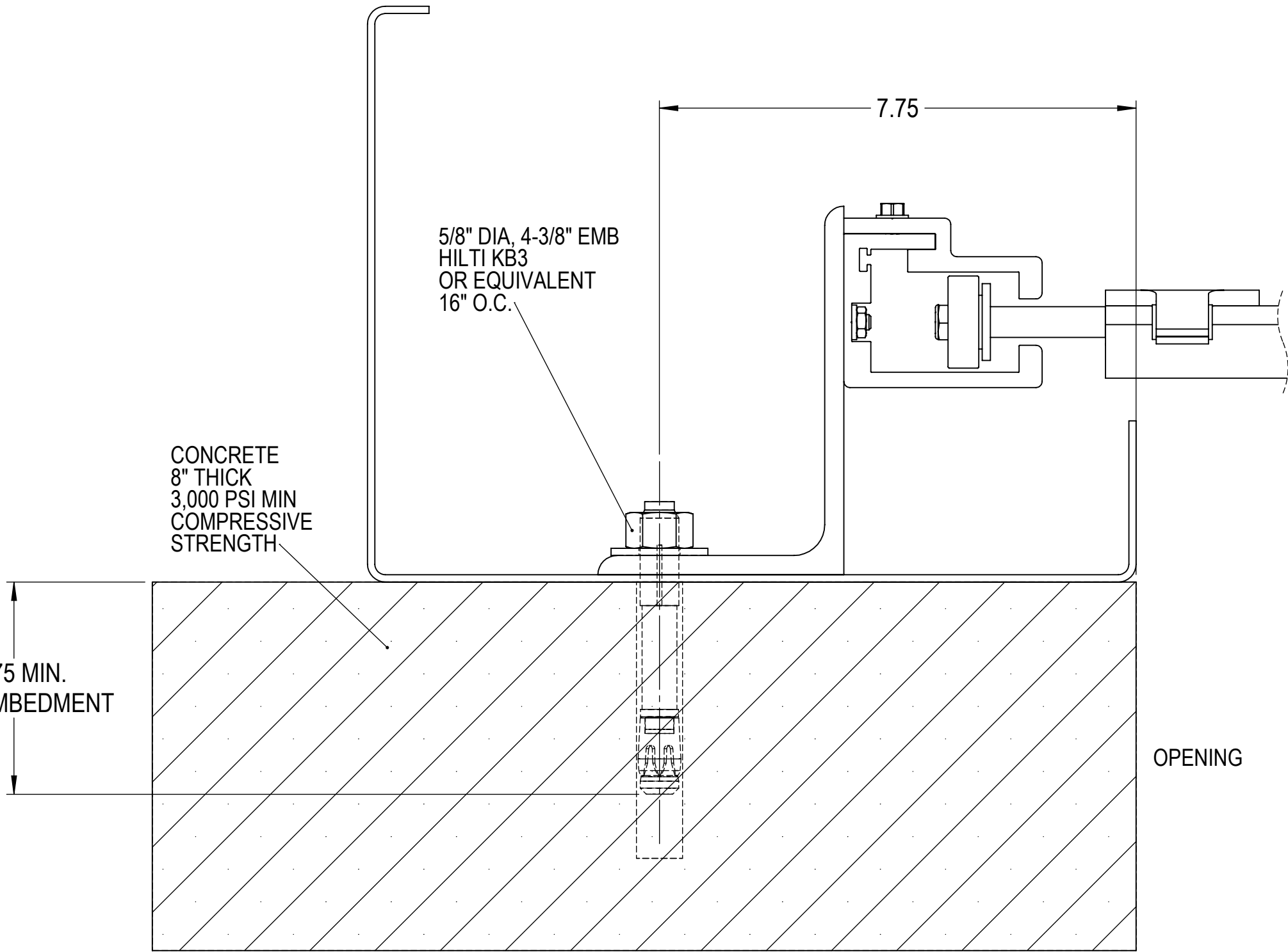
Z-GUIDE, CONCRETE JAMB
