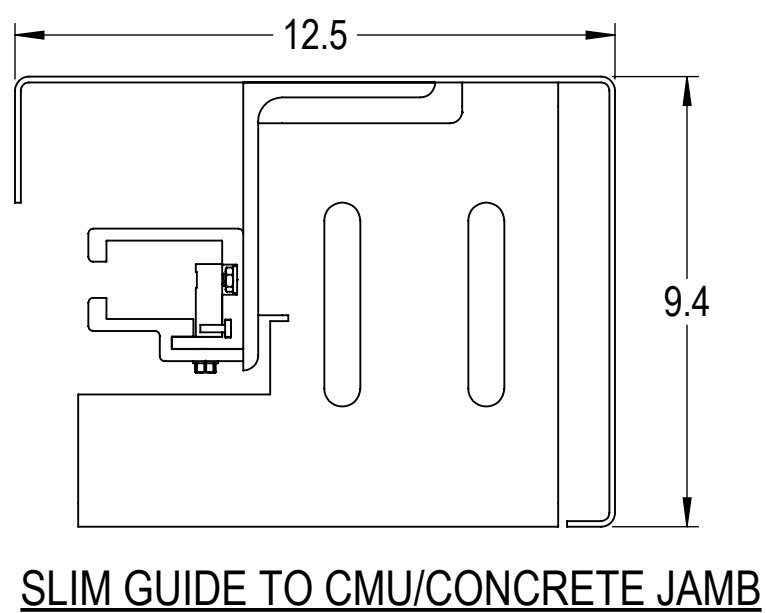
4 WALL GUIDE ASSEMBLY PROFILES (BOTTOM VIEWS)
