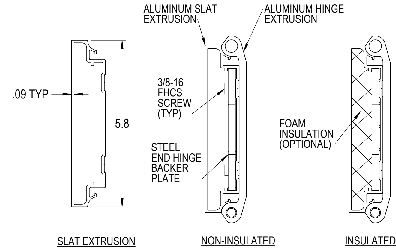
3 SLAT DETAIL
