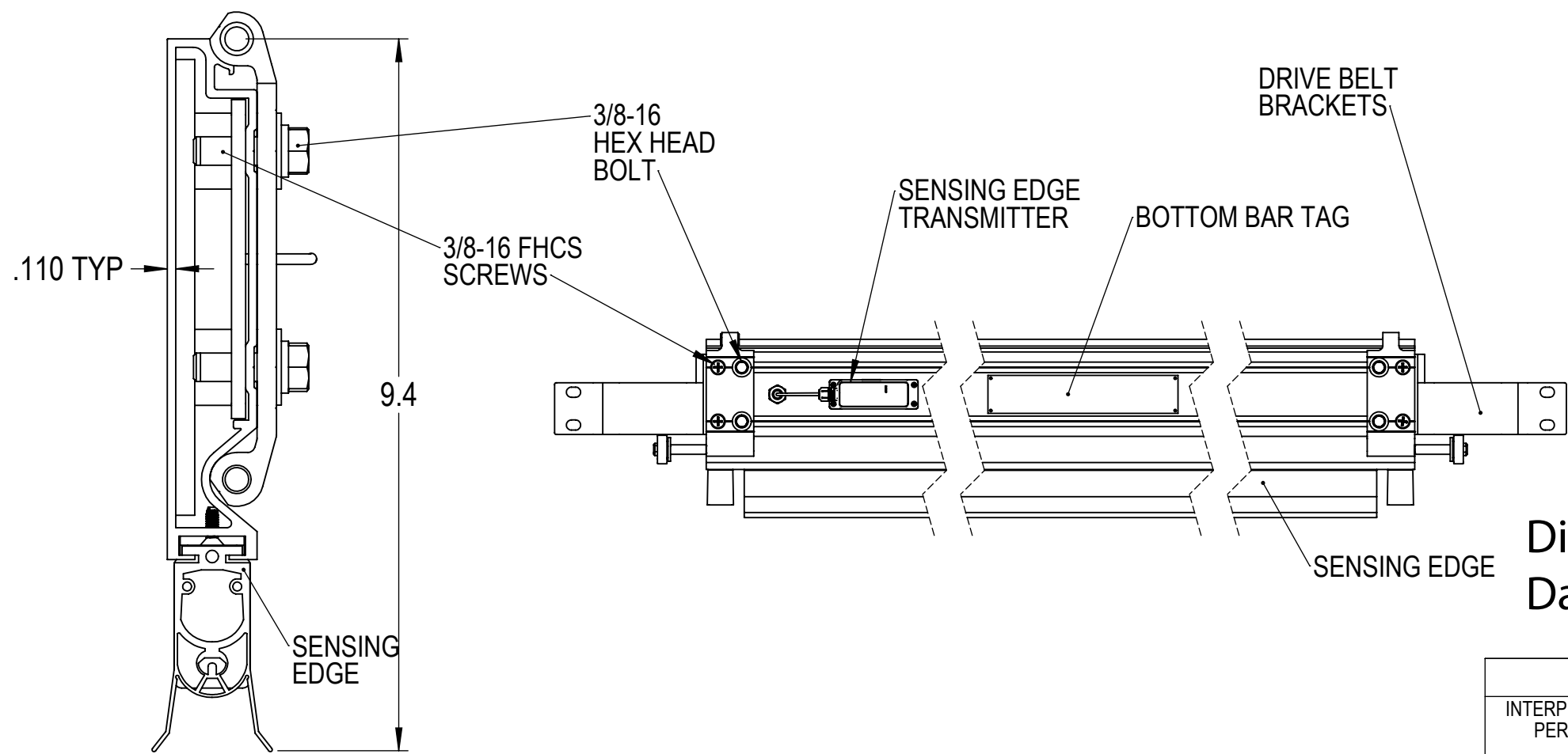
BOTTOM BAR DETAIL
